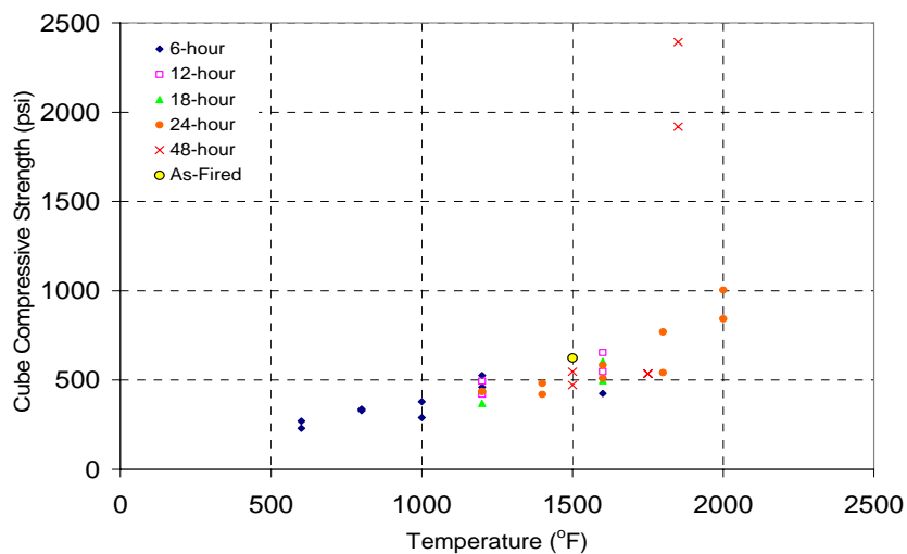
Figure 1: Effect of firing temperature and duration on compressive strengths of nominal 51-mm (2”) cubes. “As-Fired” represents the mean of the peak compressive strengths obtained for cubes cut from bricks fired in El Salvador plants.
