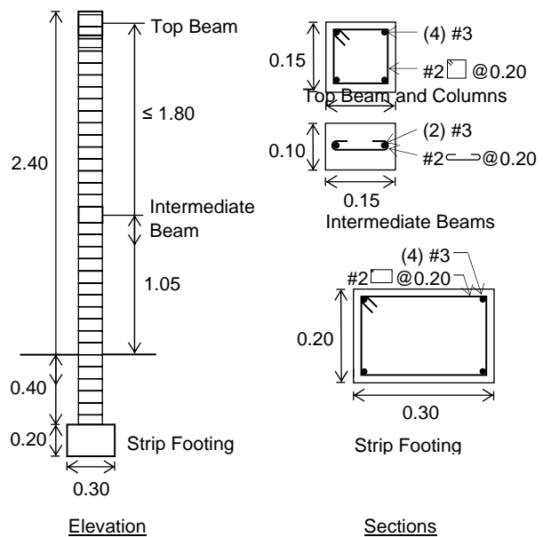
Figure 5: Typical details (reinforcing steel is in in-pound bar sizes; dimensions in meters)
