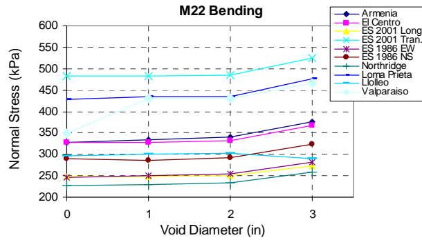
Figure 7a. Influence of void diameter on peak normal stress of out-of-plane walls (unbraced roof diaphragm)
