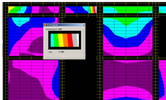
Figure 6b. Envelope values of M11 bending moment.
