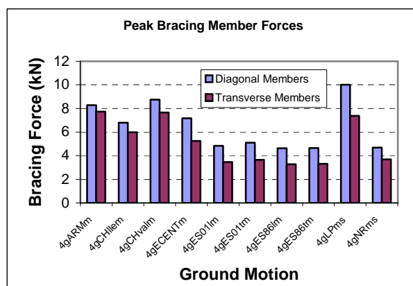
Figure 10. Bracing member forces for the solid brick model
