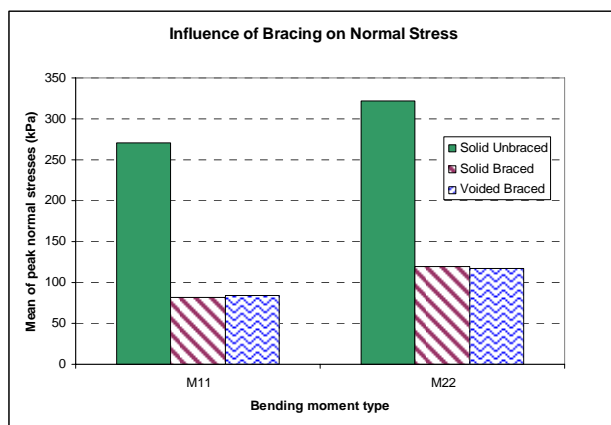
Figure 9. Influence of end-bay bracing on the average peak normal stresses.
