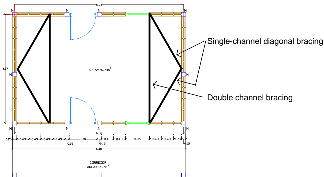
Figure 8. End-bay channel bracing
