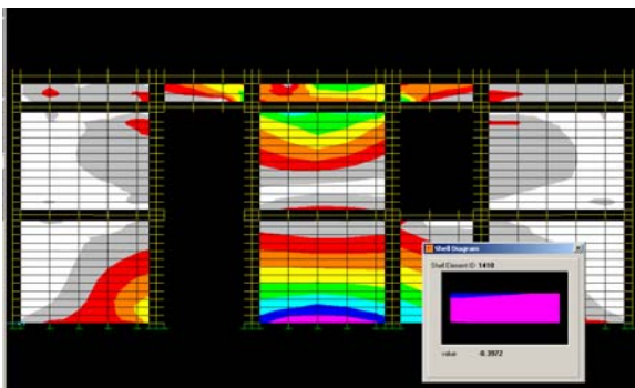
Figure 6a. Envelope values of M22 bending moment.
