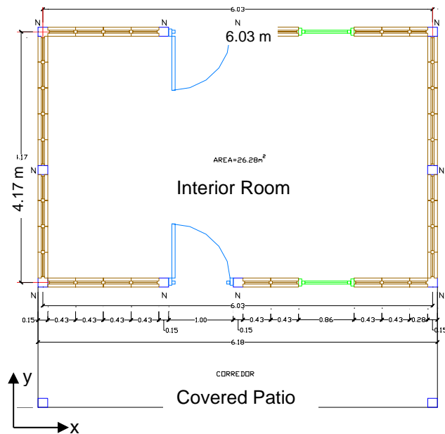
Figure 4. Plan used in analyses of mixto house.
