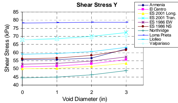
Figure 7b. Influence of void diameter on peak nominal shear stress of in-plane walls (unbraced roof diaphragm).
